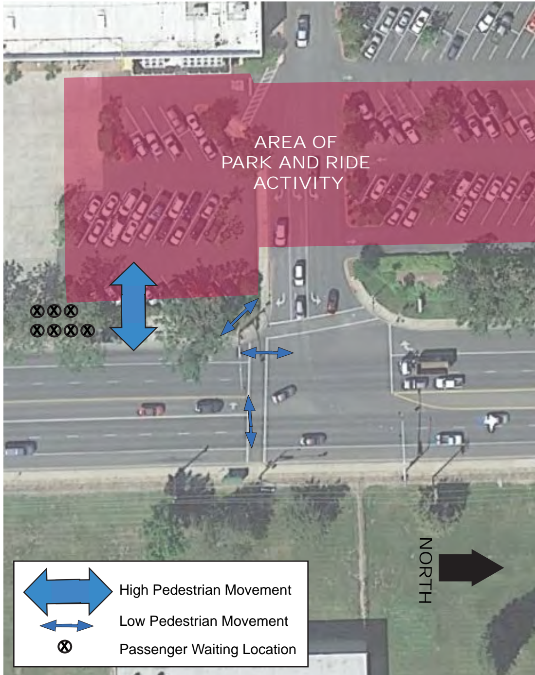
Figure 8 Walton Ave Transit Center Access Pattern
